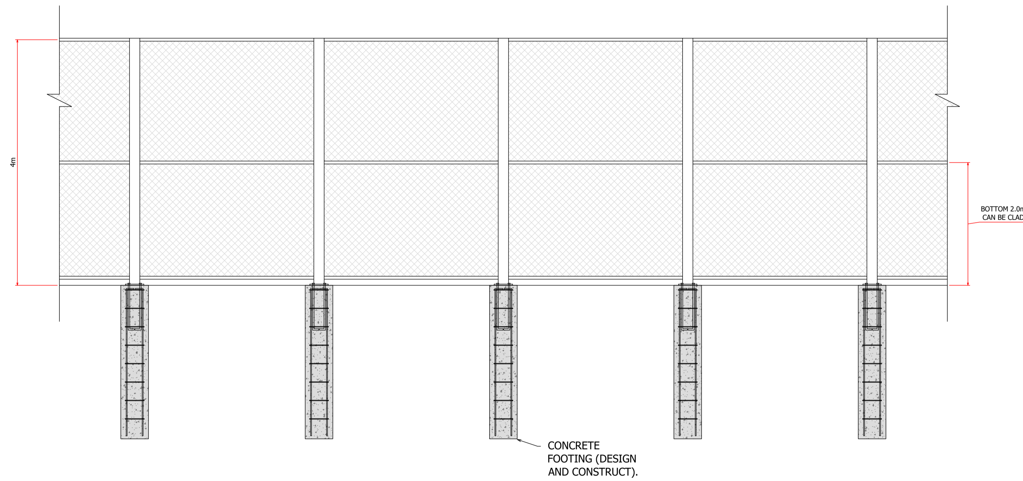
4.0m HIGH FENCE DETAIL (D&C)
