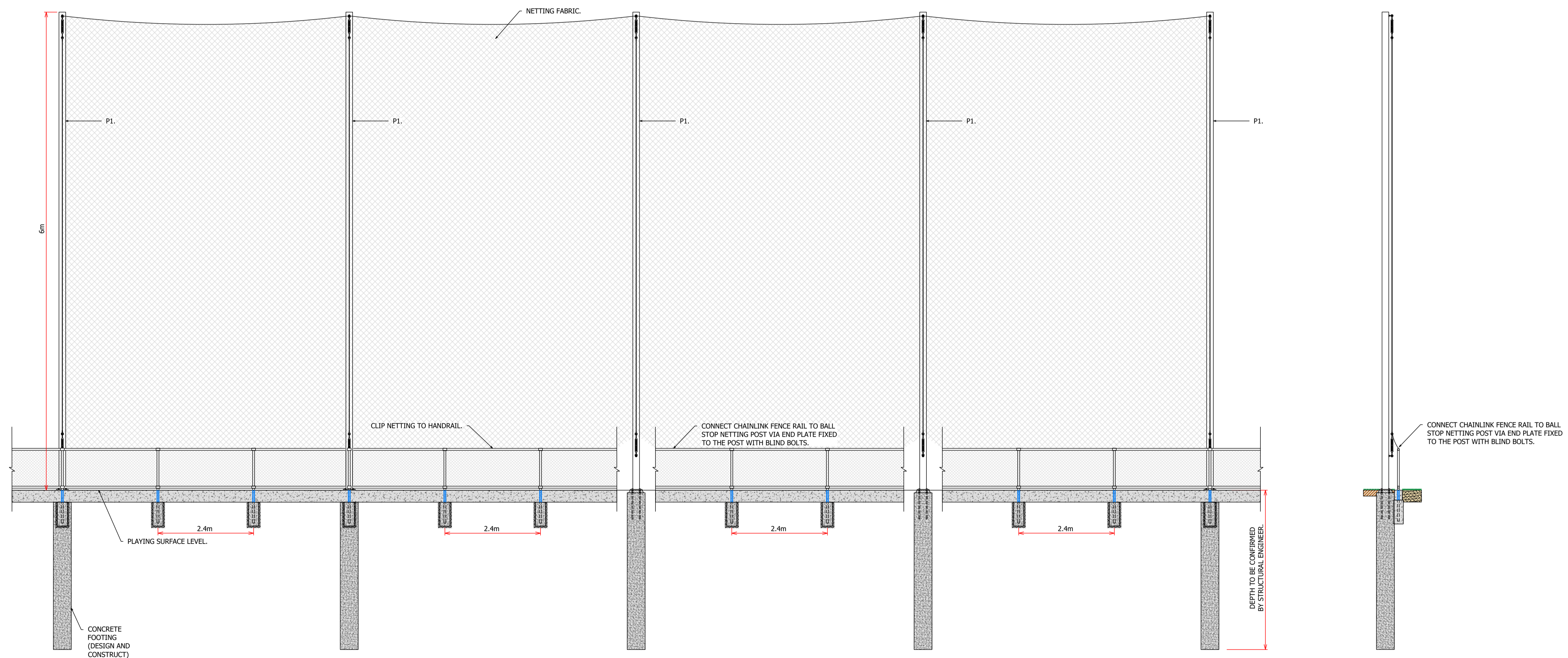
6.0m HIGH BEHIND GOAL NETTING FENCE DETAILS (D&C)
