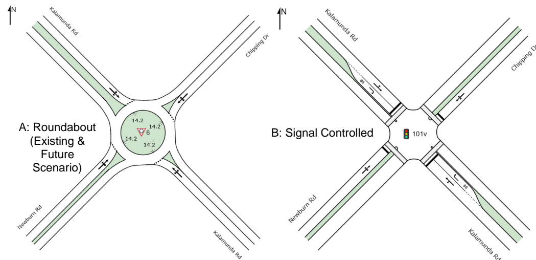
Figure 6-8 Sidra Layout for Kalamunda Road – Newburn Road/Chipping Drive Intersection
