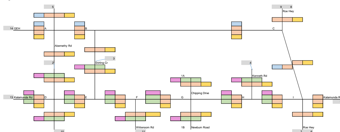
Figure 6-2 Network Model
