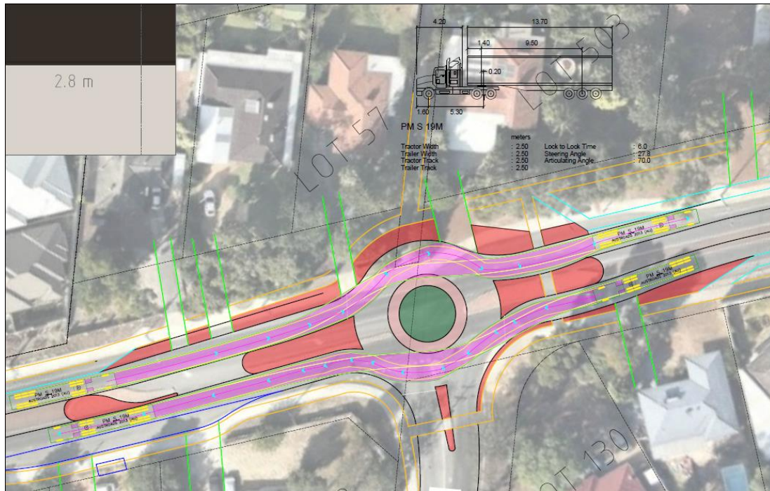
Figure 4-16 Swept path analysis at proposed Kalamunda Rd/Cyril Road intersection
