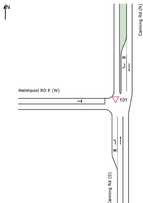
Figure 7: Canning Road / Welshpool Road E Intersection Layout
