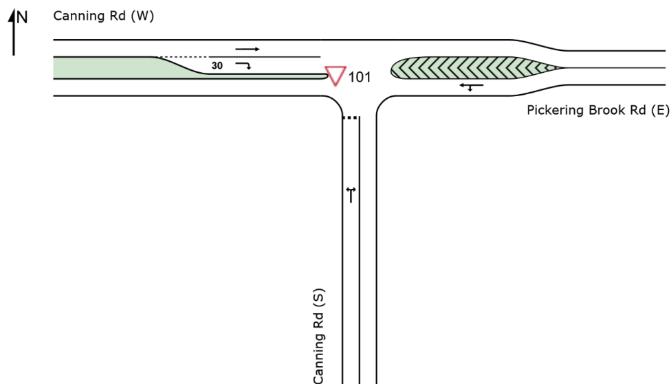
Figure 6: Canning Rd / Pickering Brook Rd. Intersection Layout
