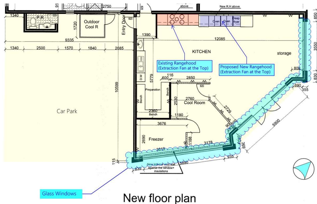
Figure 3 Proposed layout
