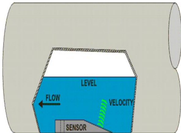
Doppler Ultra Sonic Water Sensor
