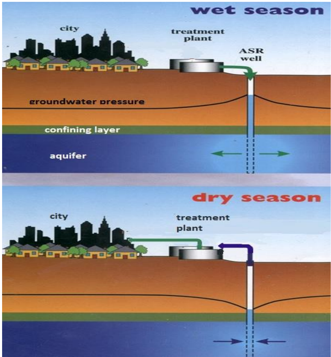
Figure 11: Schematic representation of ASR
