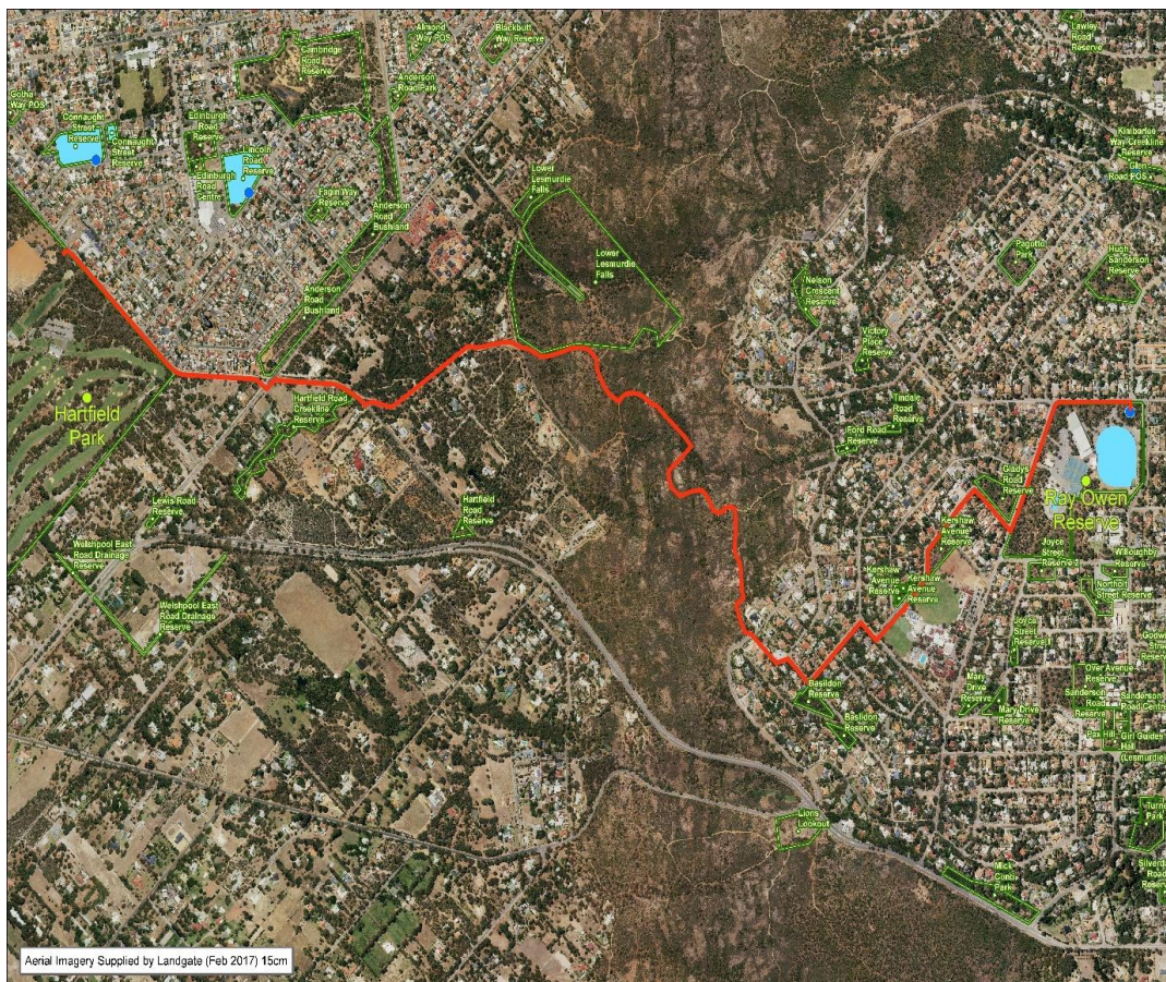
Figure 12: Proposed Pipeline Route
